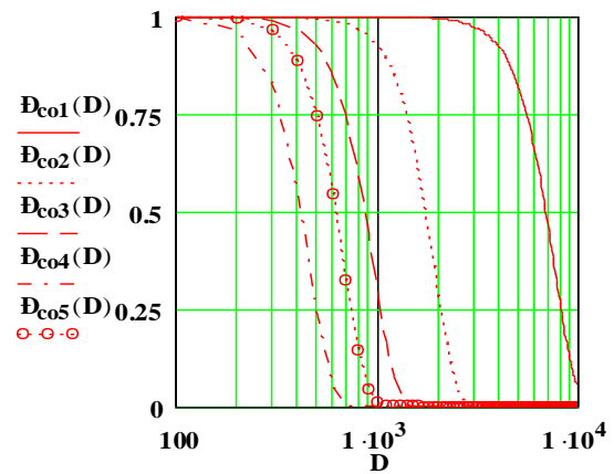
Fig. 2. Statistical probabilities of different targets detection of ZU-23 personnel P_{coi} depending on the range to them D
