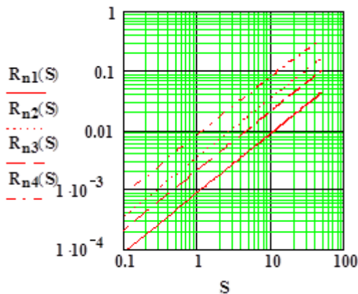
Fig. 3. Conditional probability of target destruction R_{ni}(S) depending on the area of target projection S in the image firing plane of the target
