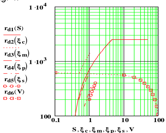
Fig. 4. Slope distances to the outedge of the engagement area r_{di} depending from S, \xi_c, \xi_m, \xi_p, \xi_s, V target
