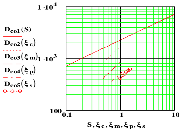
Fig.1. Target detection range D_{co} from variable S, \xi_c, \xi_m, \xi_p, \xi_s
